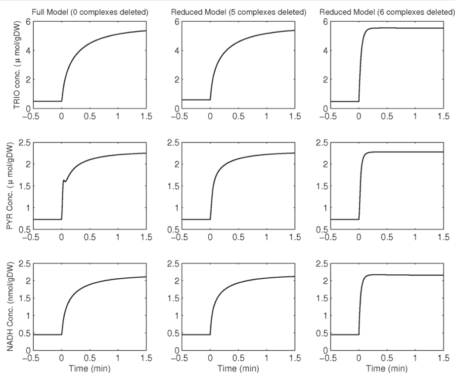
Figure 4 Comparison of concentration profiles of yeast-glycolysis metabolites between the full and reduced models.
