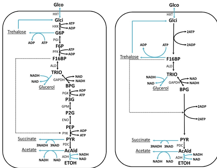
Figure 2 Schematic of the original and reduced yeast-glycolysis networks. The left-hand panel is a schematic representation of the yeast glycolysis model used for model reduction. The full model description and an explanation of all the abbreviations is found in [26]. The right-hand panel represents the reduced model after deleting 5 complexes (F6P, P2G, P3G, G6P and PEP). The blue arrows in the two panels indicate external fluxes.
