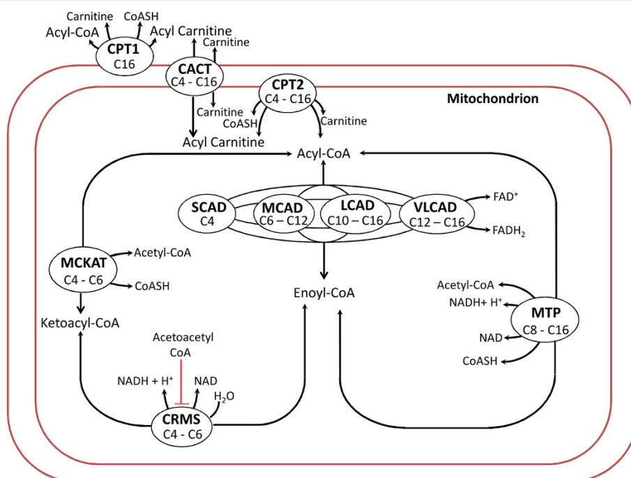
Figure 7 Schematic of the reduced model (with 12 complexes deleted) of beta-oxidation in rat liver. CRMS is a fictitious enzyme as described in the section "Fatty acid beta-oxidation model".
