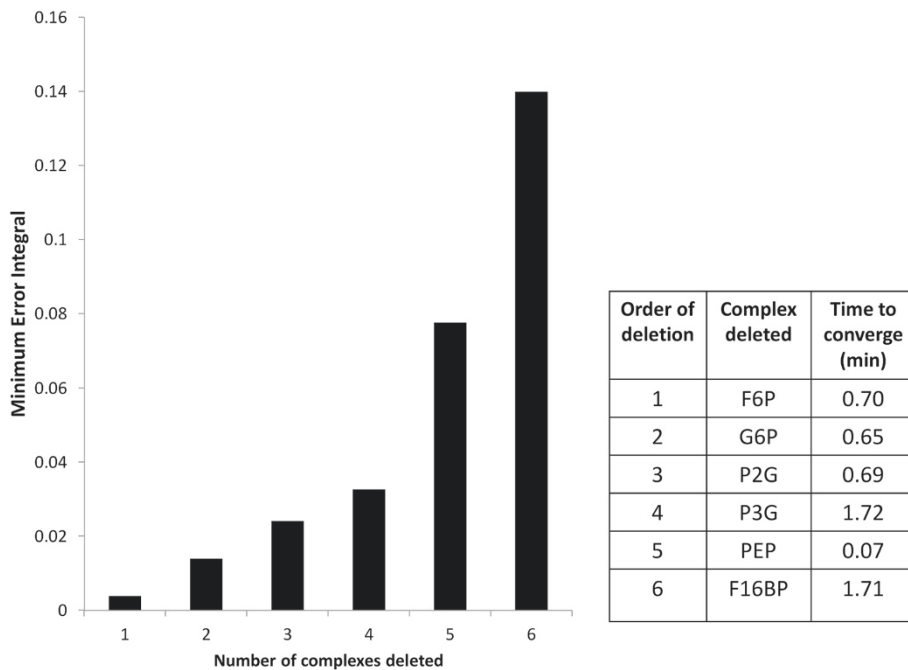
Figure 3 Reduction of the yeast glycolysis model. Left-hand panel: minimum error integral versus number of deleted complexes (we have taken T = 1.5 min for the computation of the error integral). Right-hand panel: identity of the deleted complexes and their convergence times.
