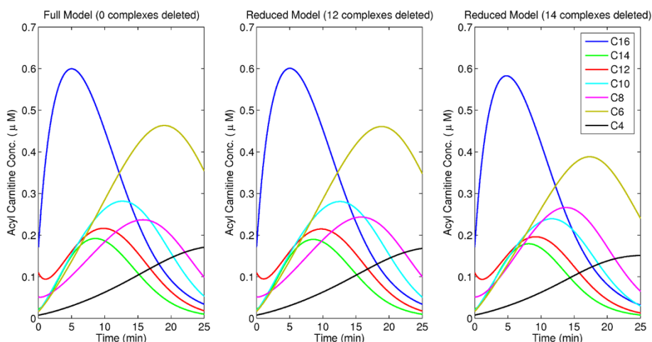
Figure 8 Comparison of concentration profiles of acyl carnitines between the full and reduced beta-oxidation models.
