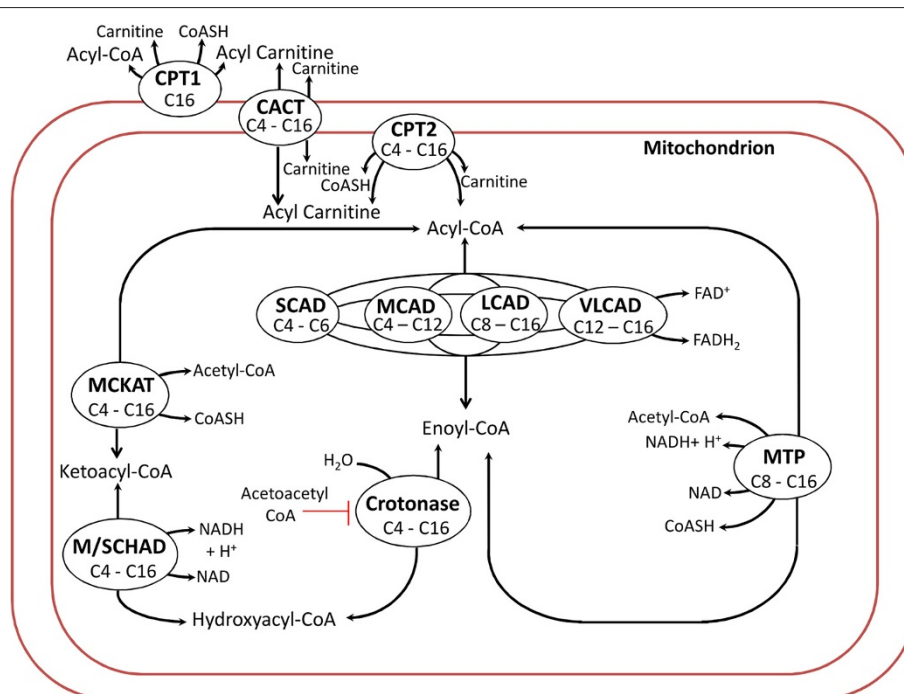
Figure 5 Schematic of a model of beta-oxidation in rat liver. The ellipses within, on and outside the boundary of the mitochondrion represent the enzymes responsible for the beta-oxidation. The full model description and explanation of all the abbreviation can be found in [27].
