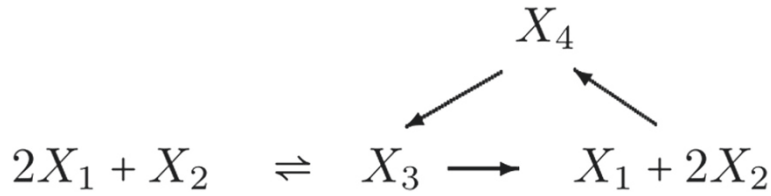
Figure 1 Example of a reaction network.
