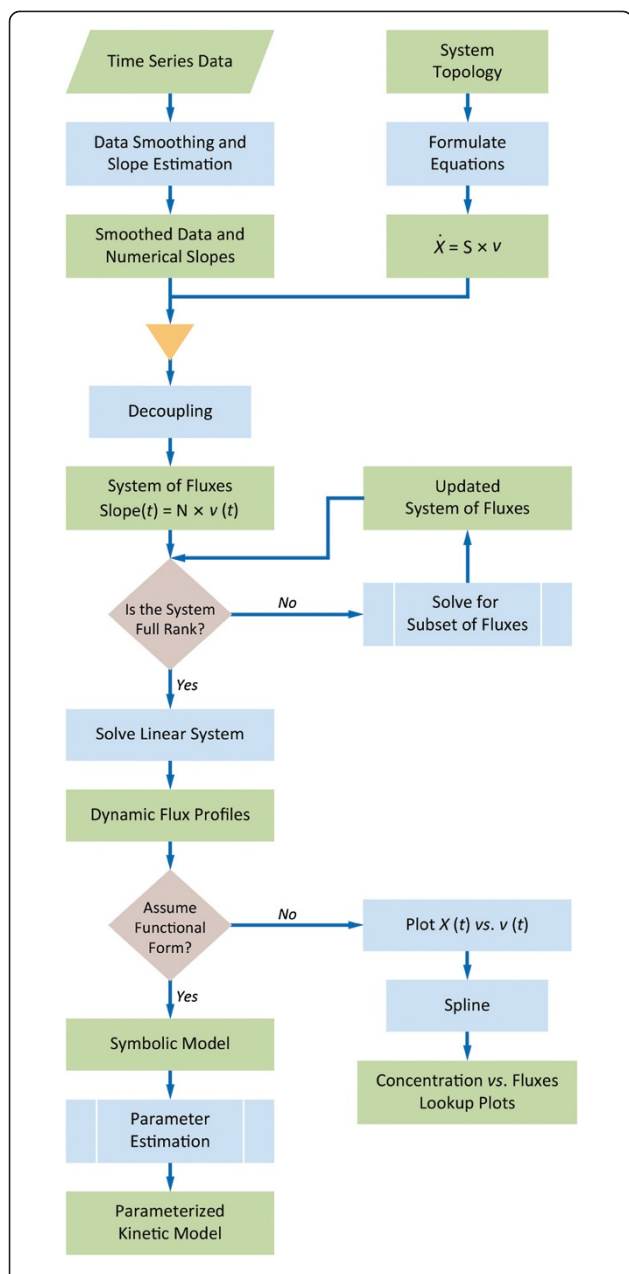
Figure 5 Flowchart of the proposed method. Starting with experimental time series, the data are smoothed and balanced for mass conservation, if necessary. The slopes of the time series at each time point are estimated. Combined with the knowledge of the system topology, substitution of the derivatives in the ODE with slope information yields a linear system of fluxes. If the system has full rank, solve the system with techniques from linear algebra. If the system is underdetermined, use auxiliary steps, as proposed in this article, to solve a subset of the fluxes until the system is of full rank. The results are the dynamic profiles of all extra- and intra-cellular fluxes in the system. If desired, make assumptions regarding the functional forms of the fluxes. These functions correspond to symbolic flux representations that can be independently fitted to the respective dynamic flux profiles and result in a fully parameterized kinetic model. As an alternative each process may be approximated as a piecewise function, for instance using spline methods.
