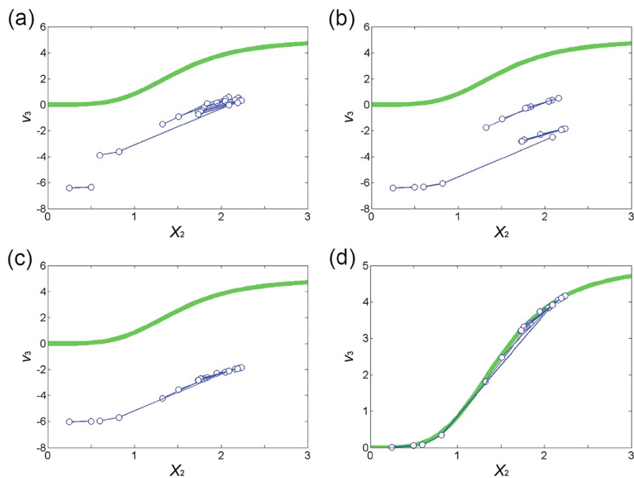
Figure 8 (a) Collection of s pieces exceeding a chosen threshold d (here s = 12 and d = 0.2 ; see Text). The green line is the “true” functional representation of X_2 versus v_3 . (b) Pairs in (a) are merged based on their distances and on the distances between two points in a pair. (c) The subgroups of pairs in (b) are merged. (d) The sigmoidal shape of points in (c) suggests that the flux of the smallest X_2 ( \sim 0.25 ) should be close to zero. The sum of errors between the estimated points and their corresponding true values (on the green line) is 0.0551.
